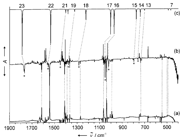
Figure 2. IR spectra illustrating the photochemistry of 5-deuterio-2,4,6-trifluoro-1,3-diodobenzene ( 4c ) in solid neon at 3 K; (a) difference spectrum; bands pointing upward increase, bands pointing downward decrease on irradiation (10 min, 254 nm); increasing absorptions are assigned to monoradical 5c ; (b) difference spectrum; bands pointing upward increase, bands pointing downward decrease on annealing the neon matrix (7.5 K, 10 min) after 16 h of irradiation with 254 nm; bands marked with ° are assigned to diradical 6c ; (c) calculated [BLYP/6-311G(d,p), unscaled] spectrum of 1,3-didehydro-5-deuterio-2,4,6-trifluorobenzene ( 6c )
