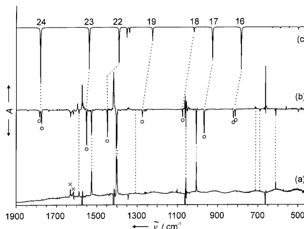
Figure 5. IR spectra illustrating the photochemistry of 1,3,5-trifluoro-2,4,6-triiodobenzene ( 4f ) in solid neon at 3 K; (a) difference spectrum; bands pointing upward increase, bands pointing downward decrease on irradiation (10 min, 254 nm); increasing absorptions are assigned to monoradical 5f ; (b) difference spectrum; bands pointing upward increase, bands pointing downward decrease on annealing the neon matrix (7.5 K, 10 min) after 16 h of irradiation with 254 nm; bands marked with ° are assigned to di-radical 6f ; (c) calculated [BLYP/6-311G(d,p), unscaled] spectrum of 1,3-didehydro-5-iodo-2,4,6-trifluorobenzene 6f
